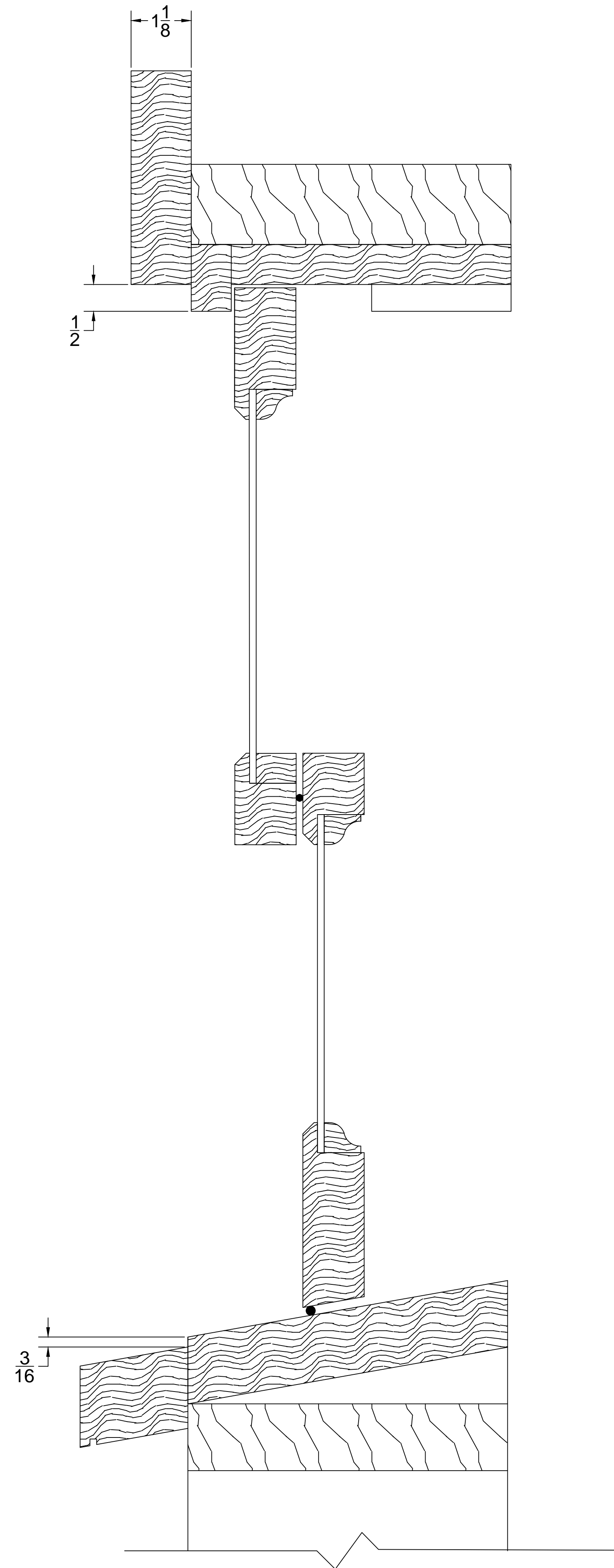
FLUSH FRAME ALUMINUM COMBINATION STORM WINDOW
